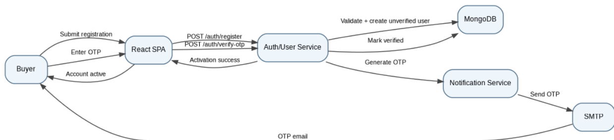
Figure 2. Registration, OTP generation, e-mail delivery and verification
