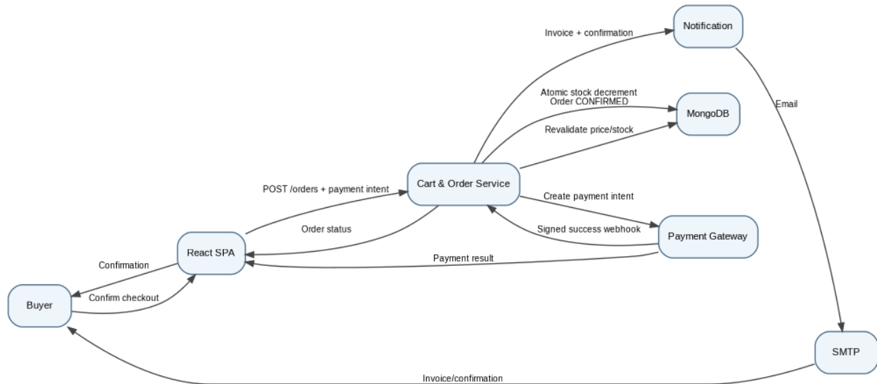
Figure 3. Checkout, payment gateway callback, stock update and notification
